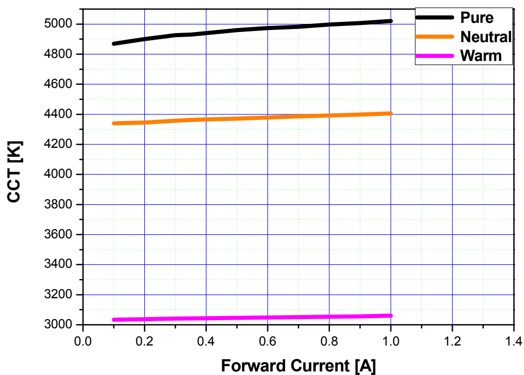
CCT vs. Forward Current, Ta=25℃
